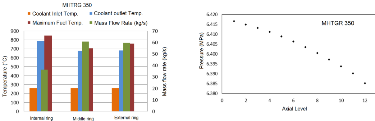
Figure 4: Left: behavior of the parameters: coolant inlet and outlet temperatures (in orange and blue), maximum fuel temperature (wine) and mass flow rate (green); Right: pressure behavior along any THC of the MHTGR350 MW.
