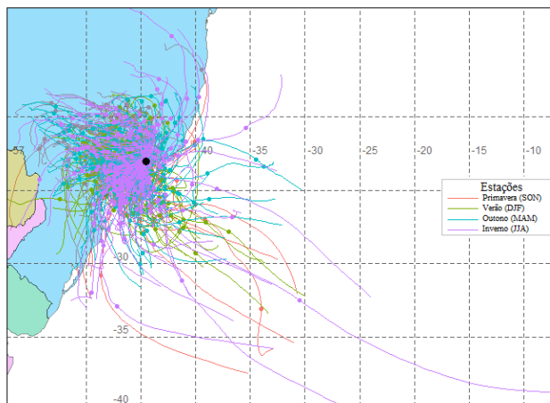
3.1 - Daily seasonal radionuclide trajectories identified by colors from the Angra 1 and Angra 2 plants with 72-hour dispersion for 2019 with the beginning of dispersion at 00 UTC.
