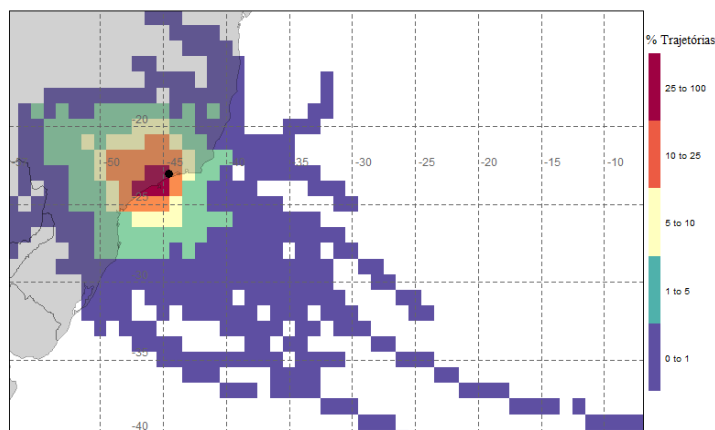
Figure 3.2 - Frequency map of daily trajectories calculated for 72 hours for the year 2019 with initial dispersion at 00 UTC from the Angra 1 and Angra 2 plants.
