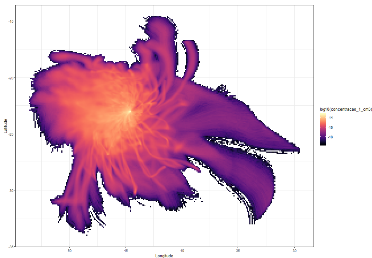
Figure 3.3 - Concentration log map for daily 48-hour dispersions for 2019 starting at 00 UTC from the Angra 1 and Angra 2 plants.
