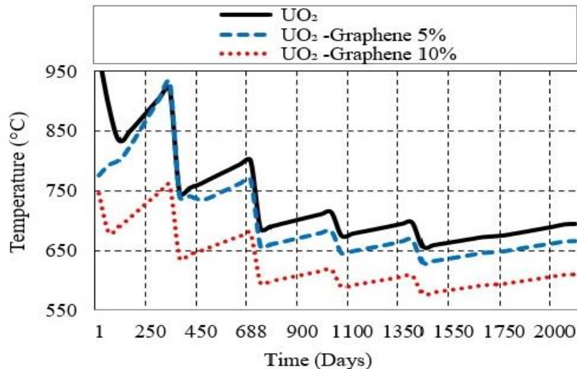
Figure 1: Fuel average temperature for \text{UO}_2 -5 vol% Graphene and \text{UO}_2 10 vol% Graphene
